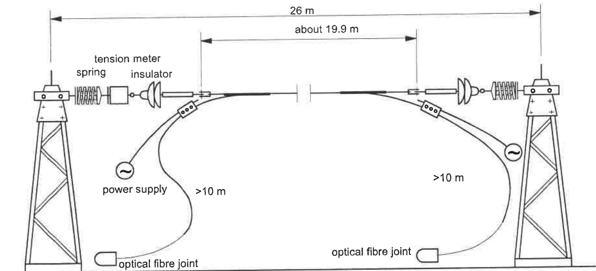
Figure 1: Test arrangement.
